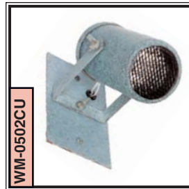
WM-0502CU MAXISPOTTER LO2036 20W MR-16 Copper & Brass Dimensions: 4.25" x 2"
