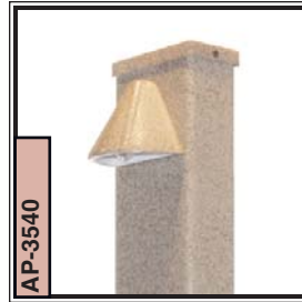
AP-3540 La PALMA LO921 16.5W Wedge Base Cast Aluminum & Phosphatized Steel Dimensions: 40.0" x 4.0"
