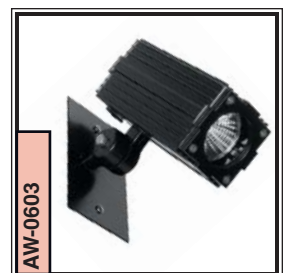
AW-0603 STYLIST LO2036 20W MR-16 Extruded Aluminum & Steel Dimensions: 5.5" x 2.5"
